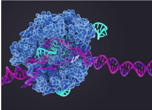
Schematic representation of Cas9-sgRNA and target DNA complex
